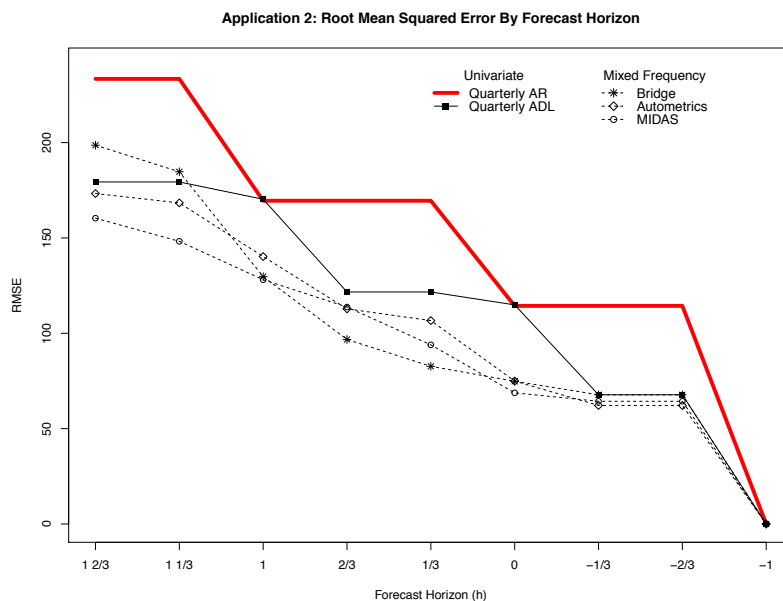
Figure 5: RMSE for each model for forecast horizons between h = 1\frac{2}{3} and h = -1 .
