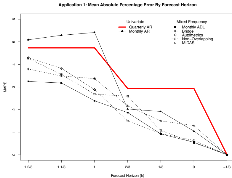
Figure 4: MAPE for each model for forecast horizons between h = 1\frac{2}{3} and h = 0 .
