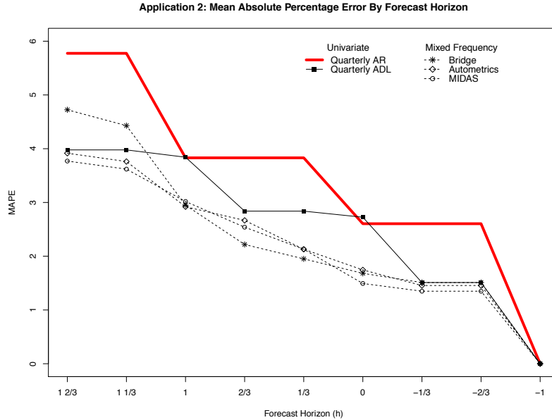
Figure 6: MAPE for each model for forecast horizons between h = 1\frac{2}{3} and h = -1 .
